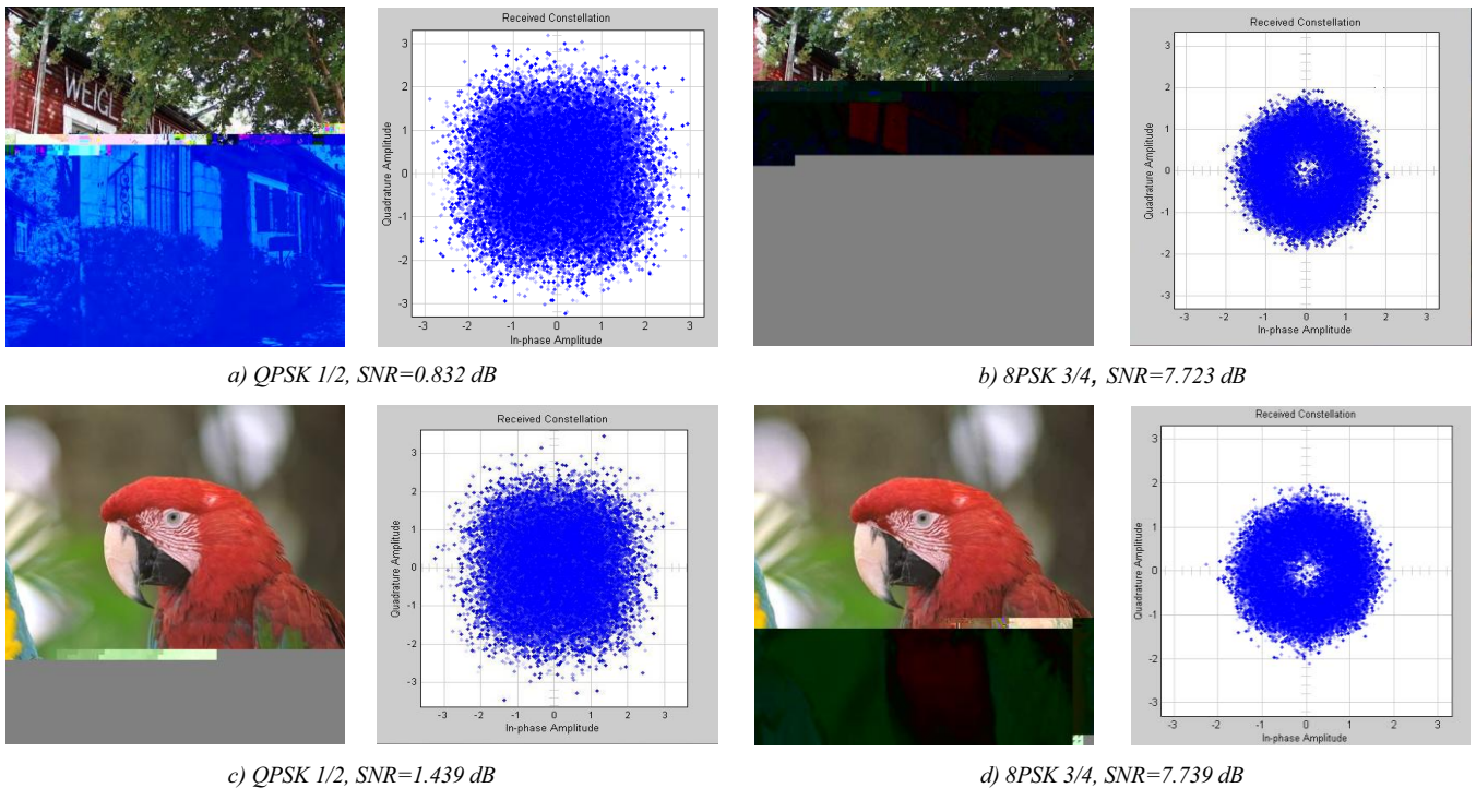
Figure 2. Simulation examples of received image and constellation diagram for two different modulations
